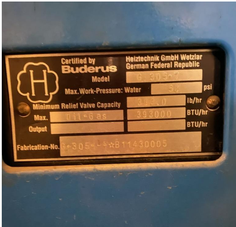
Image 2: Name plate from boiler.
